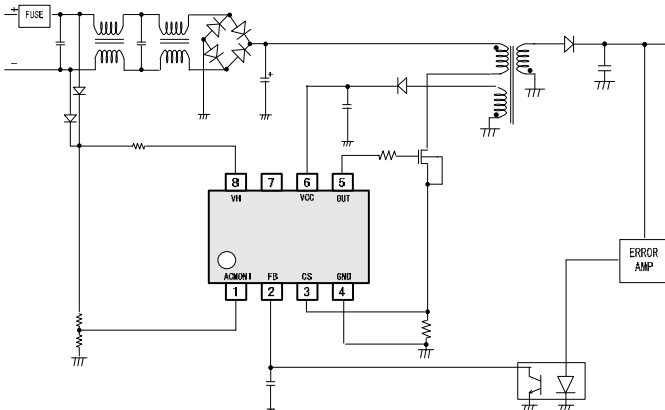
Figure 1. Application Circuit
