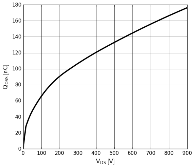
Figure 7. Typical Q_{oss}
