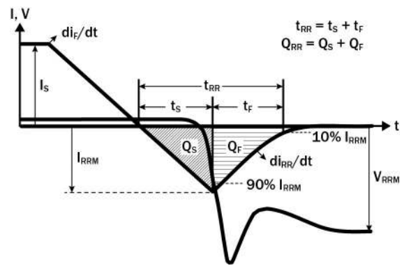
Figure 13. Diode Recovery Waveform
