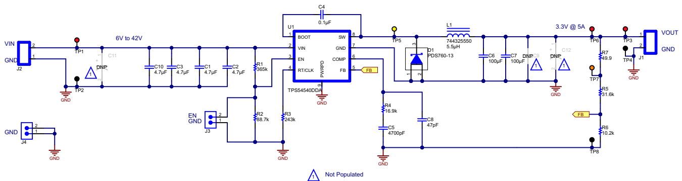
Figure 2. TPS54540EVM-558 Schematic
