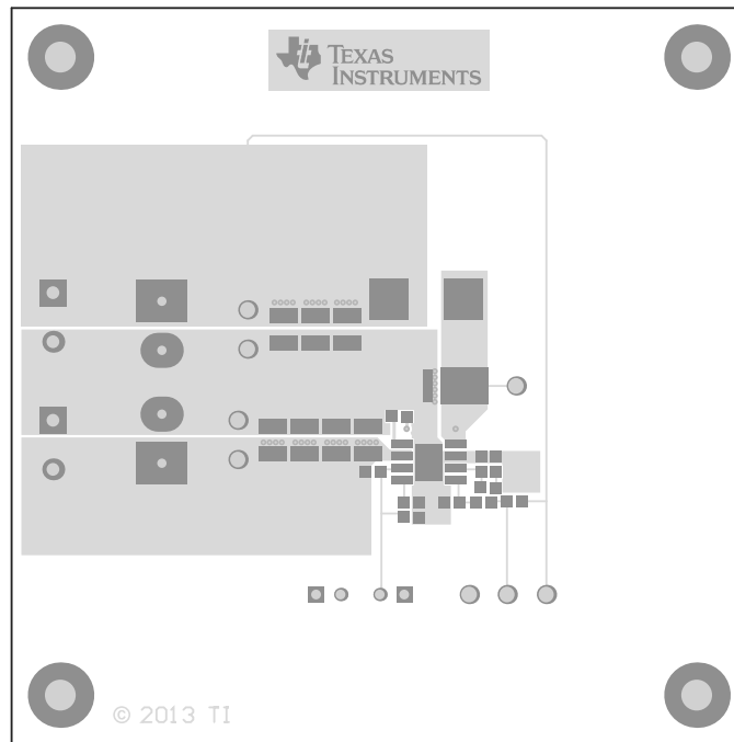
Figure 23. TPS54540EVM-558 Top-Side Layout
