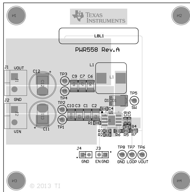
Figure 22. TPS54540EVM-558 Top Assembly and Silkscreen
