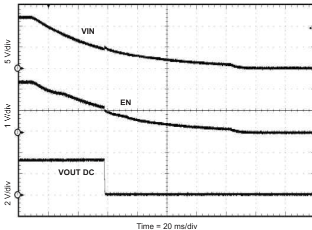
Figure 18. Shutdown Relative to V_{IN}
