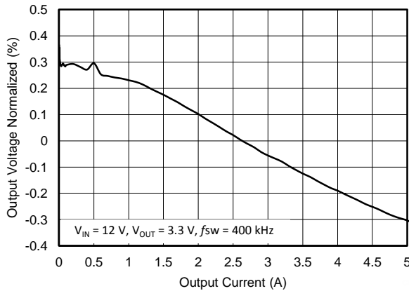
Figure 5. Regulation Versus Output Current
