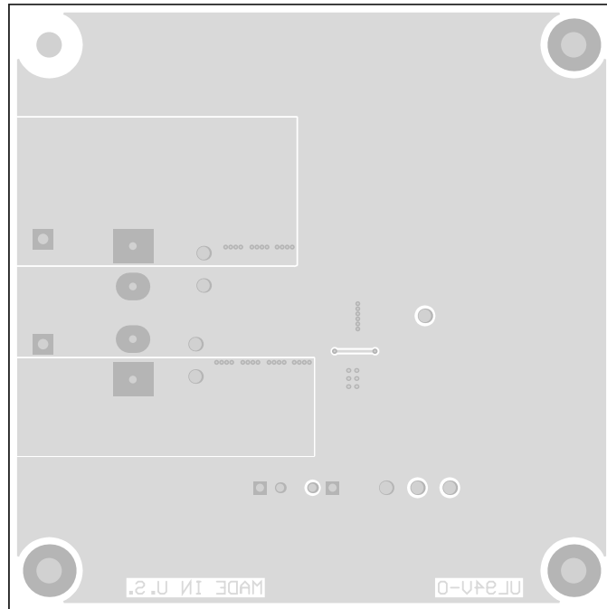
Figure 26. TPS54540EVM-558 Bottom-Side Layout
