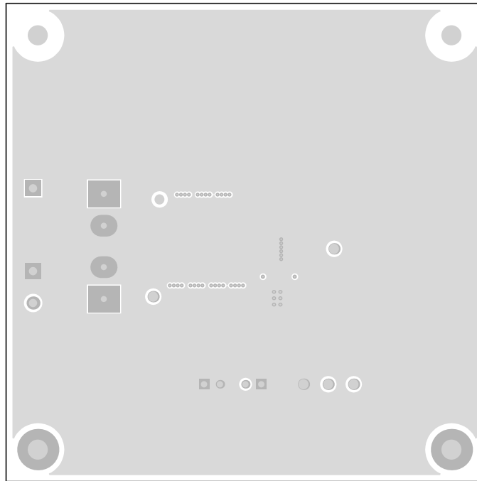
Figure 25. TPS54540EVM-558 Layer 3 Layout
