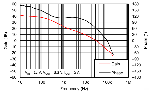
Figure 8. Loop Response
