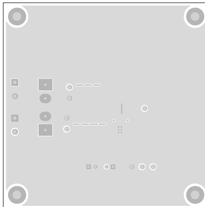
Figure 24. TPS54540EVM-558 Layer 2 Layout
