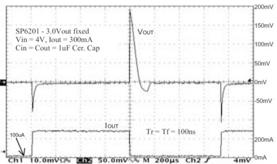
Fig. 35: Load Transient Response, 300mA step, 4V IN
