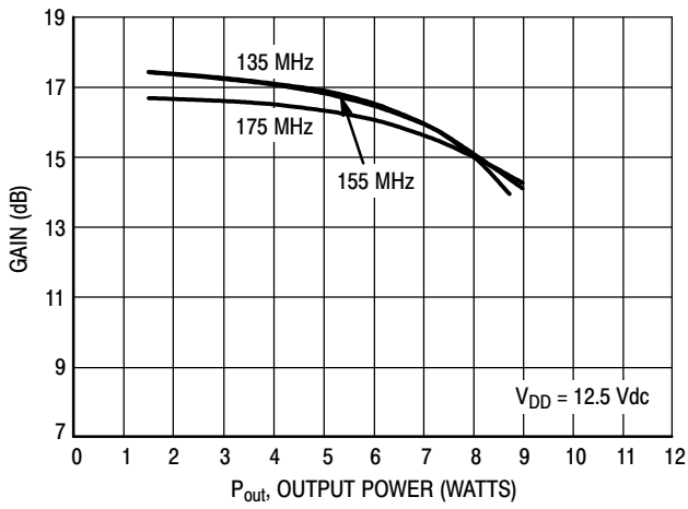
Figure 31. Gain versus Output Power
