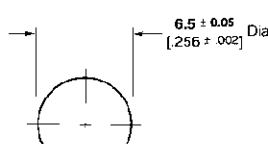
BMB Mount
