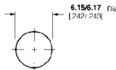
BMA Mount
