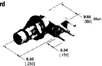
Part No. 448089-1
