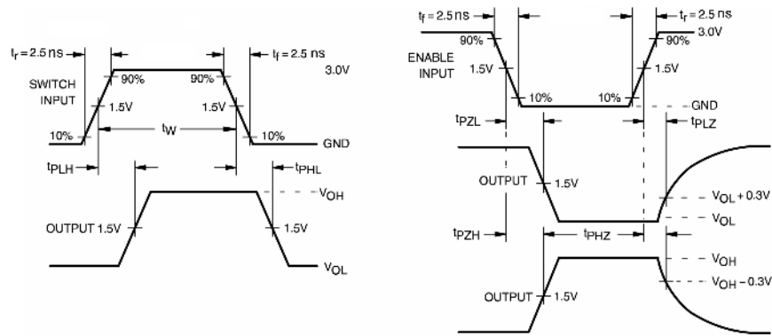
FIGURE 2. AC Waveforms
