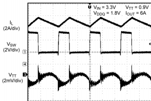
Switching Waveforms; I OUT = 6A
