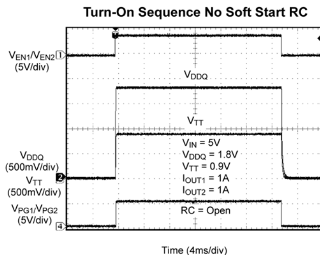
Figure 7. V_{TT} Turn-On without Delay
