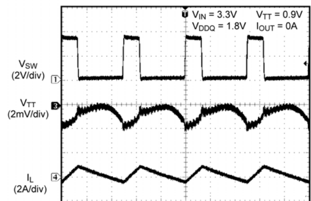
Switching Waveforms; I OUT = 0A
