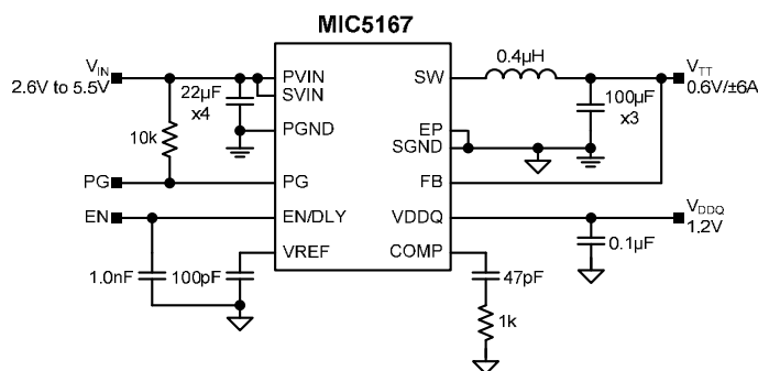
MIC5167 ±6A Synchronous Buck DDR Terminator
