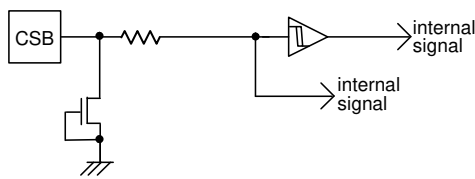
Figure 53. CSB input equivalent circuit
