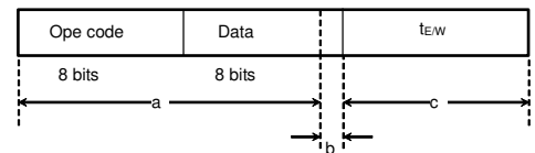
Figure 47. WRSR cancel valid timing
