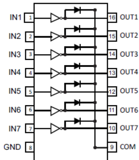
SO-16 (Type SM)
