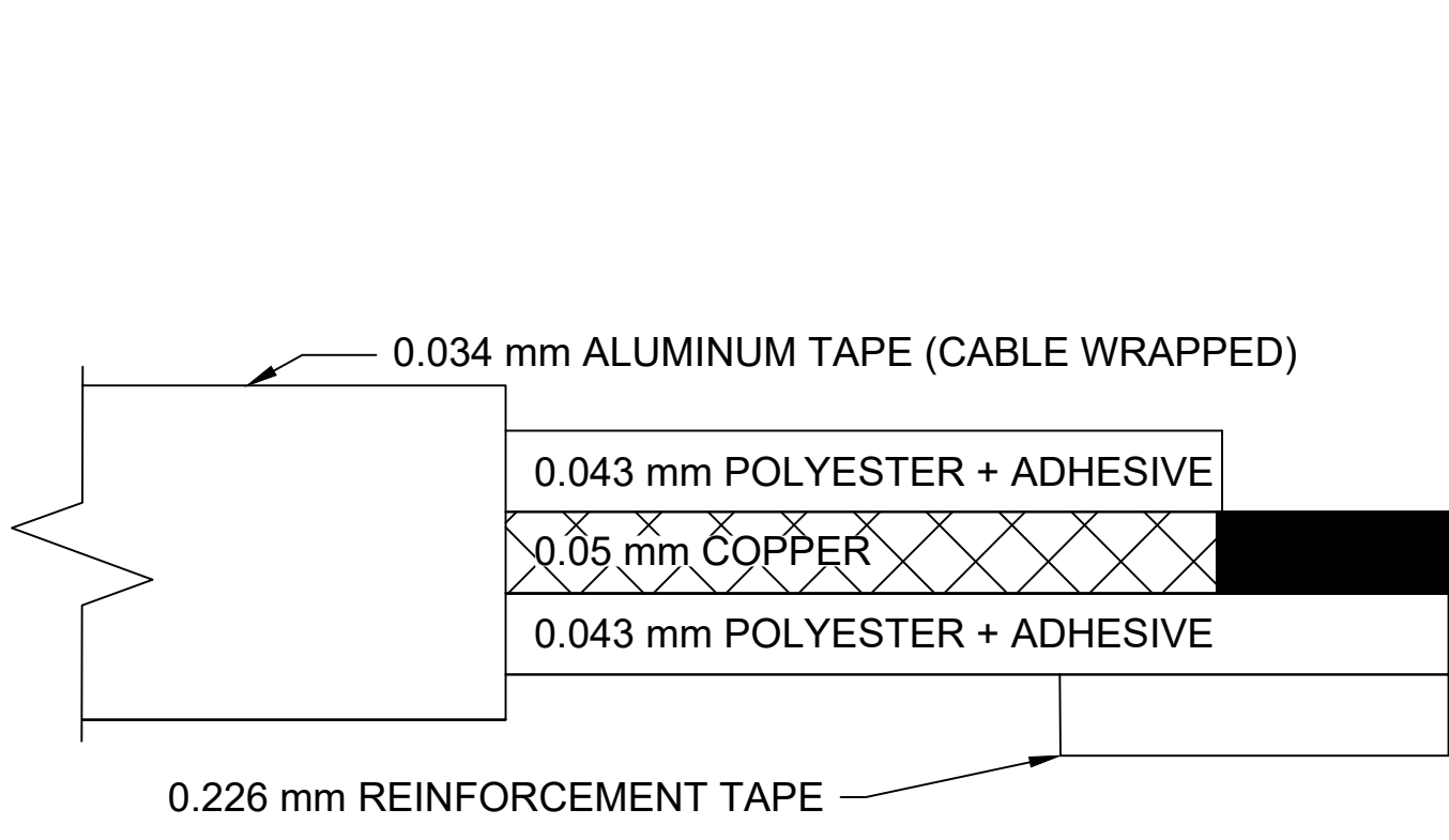
CROSS-SECTION
