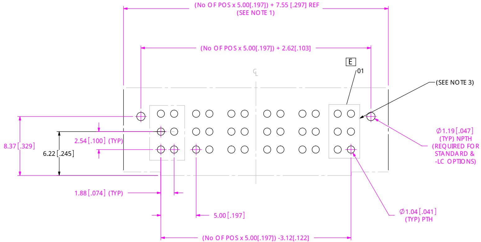
FIG. 1 PCB LAYOUT FOR MPT-XX-06.30-XX-X-VT-LC SHOWN
