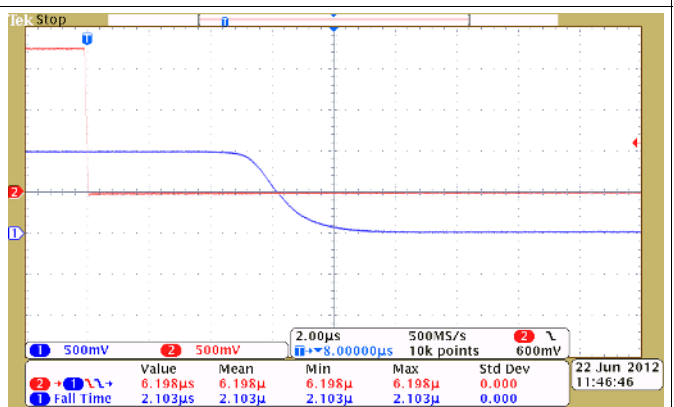
Figure 28. Turn off Response Time ( V_{IN} = 1\text{ V} , C_{IN} = 1\ \mu\text{F} , C_L = 0.1\ \mu\text{F} , R_L = 10\ \Omega )
