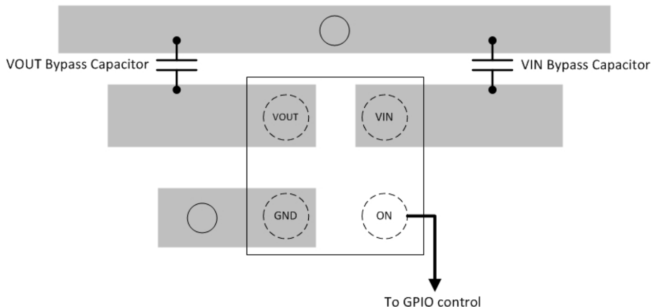
Figure 32. Layout Example
