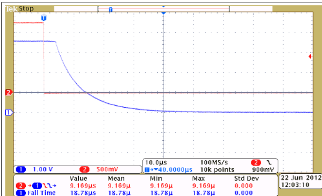
Figure 25. Turn off Response Time ( V_{IN} = 3.6\text{ V} , C_{IN} = 10\ \mu\text{F} , C_L = 1\ \mu\text{F} , R_L = 10\ \Omega )
