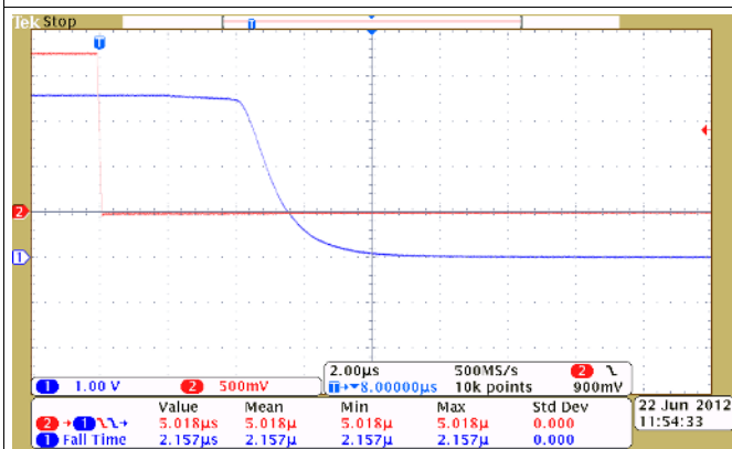
Figure 27. Turn off Response Time ( V_{IN} = 3.6\text{ V} , C_{IN} = 1\ \mu\text{F} , C_L = 0.1\ \mu\text{F} , R_L = 10\ \Omega )
