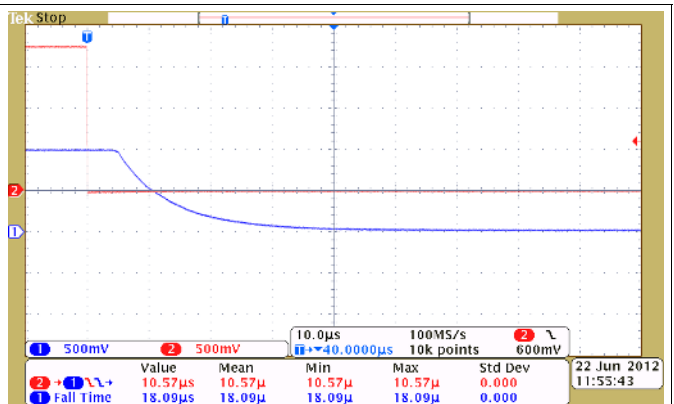
Figure 26. Turn off Response Time ( V_{IN} = 1\text{ V} , C_{IN} = 10\ \mu\text{F} , C_L = 1\ \mu\text{F} , R_L = 10\ \Omega )
