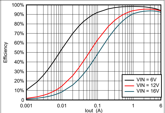
Figure 6-18. TPS566247 Efficiency at 5 V_{OUT} with a 2.2- \mu\text{H} Inductor
