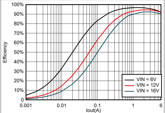
Figure 6-16. TPS566247 Efficiency at 3.3 V_{OUT} with a 2.2- \mu\text{H} Inductor
