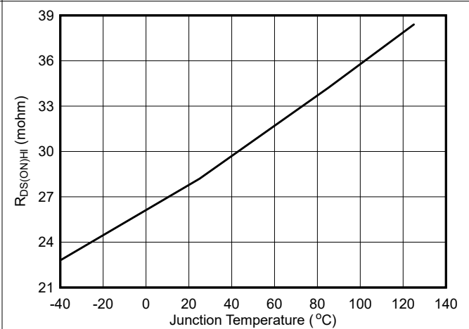
Figure 6-6. High-Side R_{DS(ON)}
