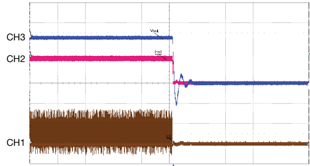
Fig. 18 - Shut-Down, I OUT = 6 A CH1 (BRN) = LX (10 V/div), CH3 (BLU) = V OUT (0.5 V/div), CH2 (RED) = I COIL (5 A/div), Time = 200 μs/div
