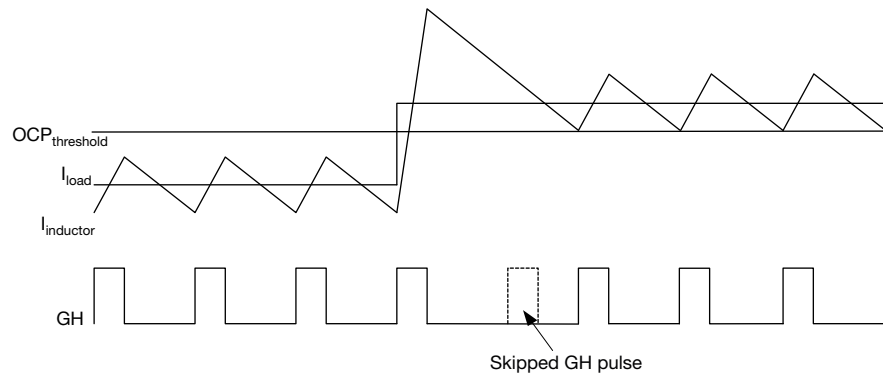
Fig. 22 - Over-Current Protection Illustration
