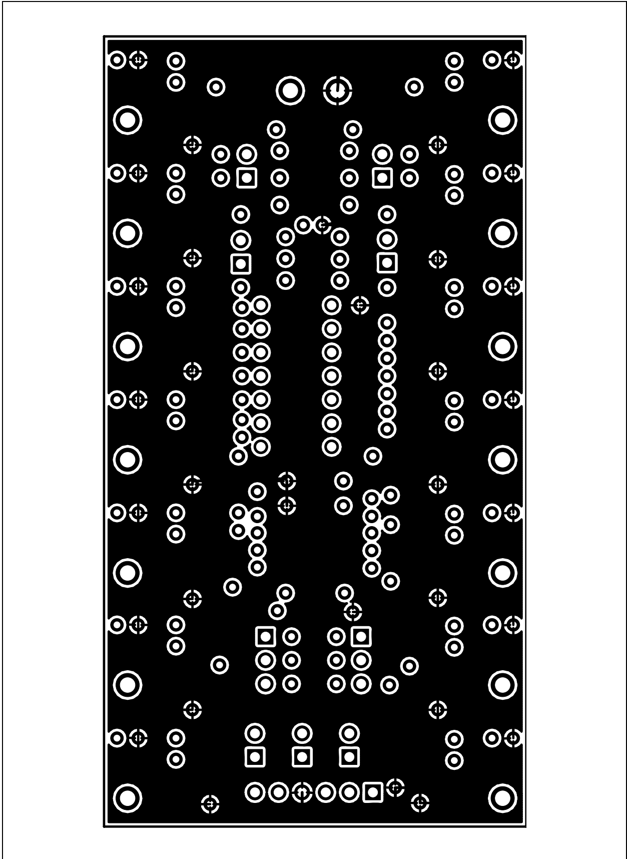
FIGURE A-7: Board Layout – Power Plane.
