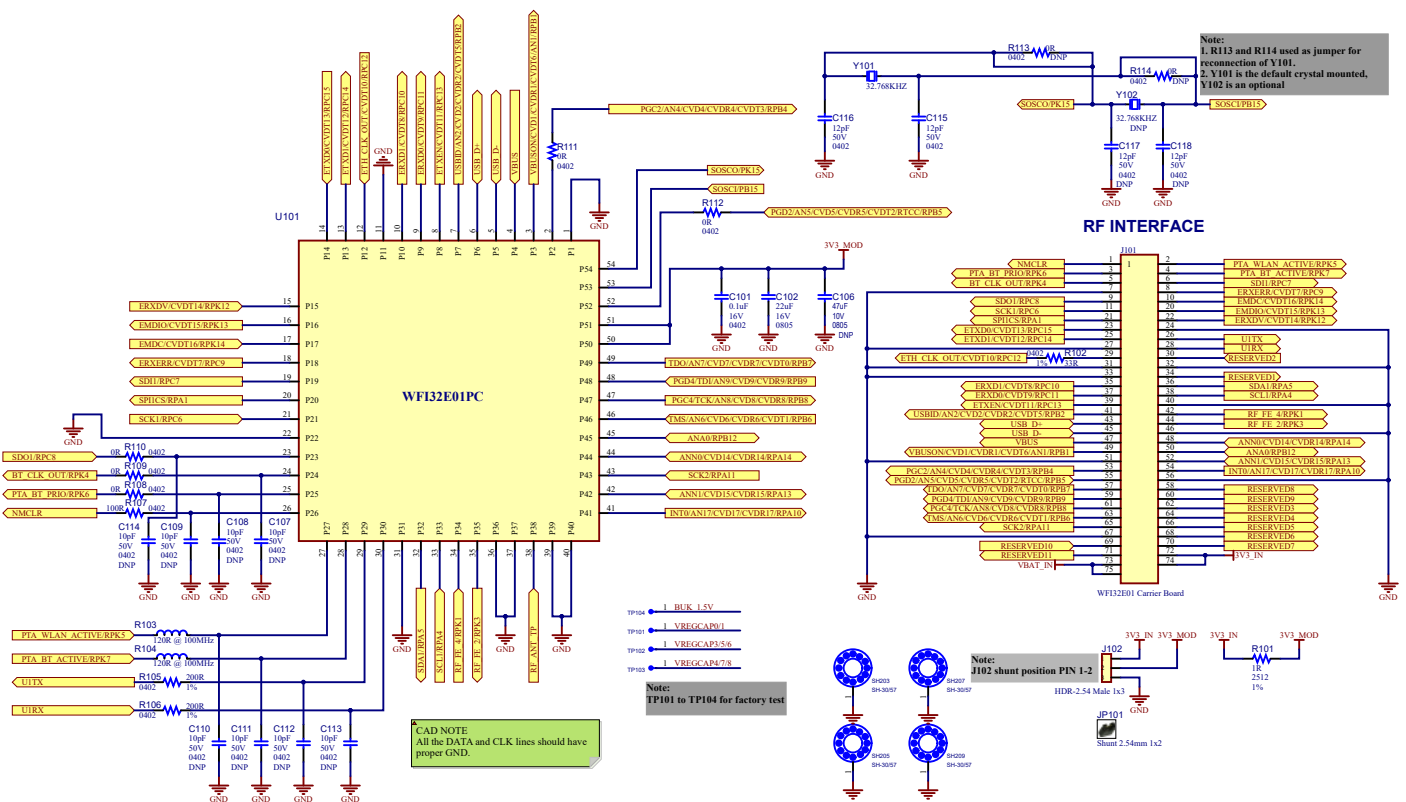
Figure 6-4. WFI32E01 Carrier Board Schematics (Sheet 4 of 4)
