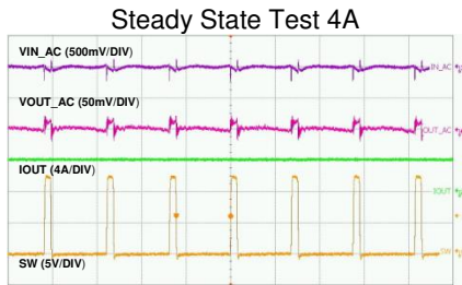
Time-1 \mu\text{s}/\text{div}
