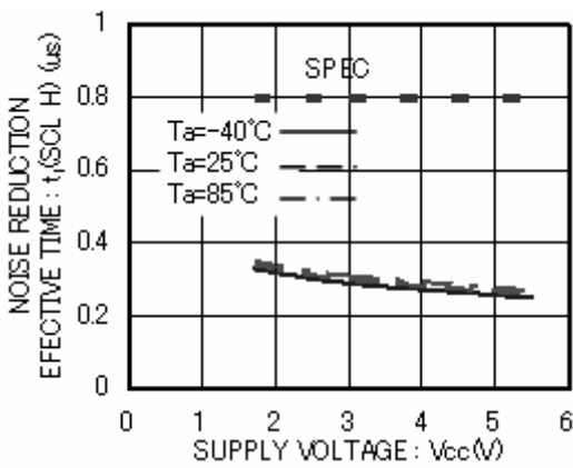
Figure 24. Noise reduction effective time t_I(\text{SCL H})
