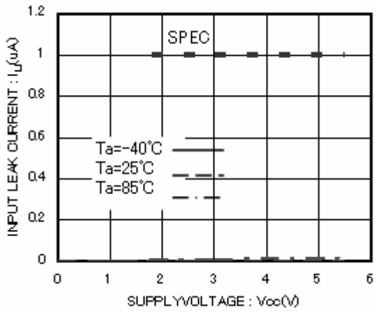
Figure 6. Input leak current I_i (A0,A1,A2,SCL,WP)
