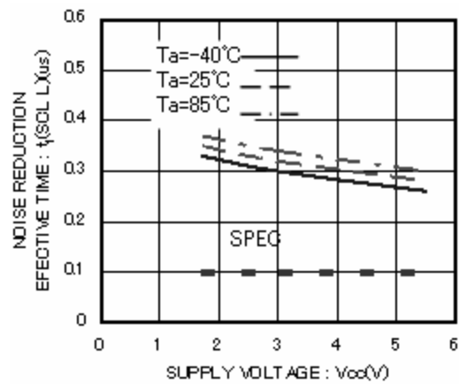
Figure 25. Noise reduction effective time t_I(\text{SCL L})
