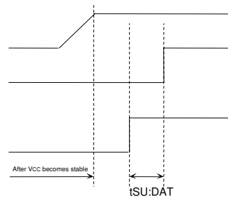
Figure 49. When SCL='H' and SDA='H'
