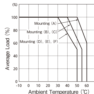
ZWS100AF Output Derating
