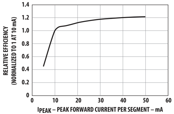
Figure 4. Relative efficiency (luminous intensity per unit current) vs. peak current.
