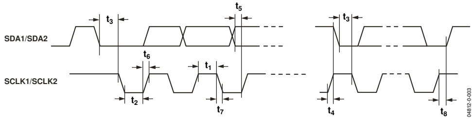
Figure 3. I 2 C Timing
