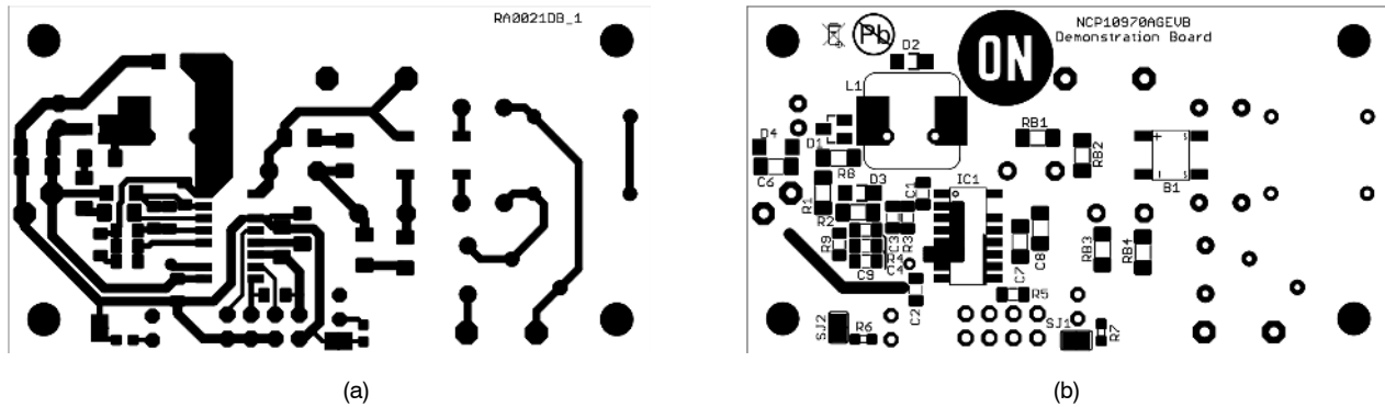
Figure 3. NCP10970AGEVB – Bottom Side – (a) Layer, (b) Components
