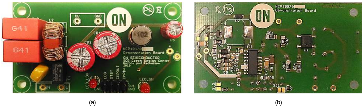
Figure 4. NCP10970AGEVB Board Photo – (a) Top Side, (b) Bottom Side
