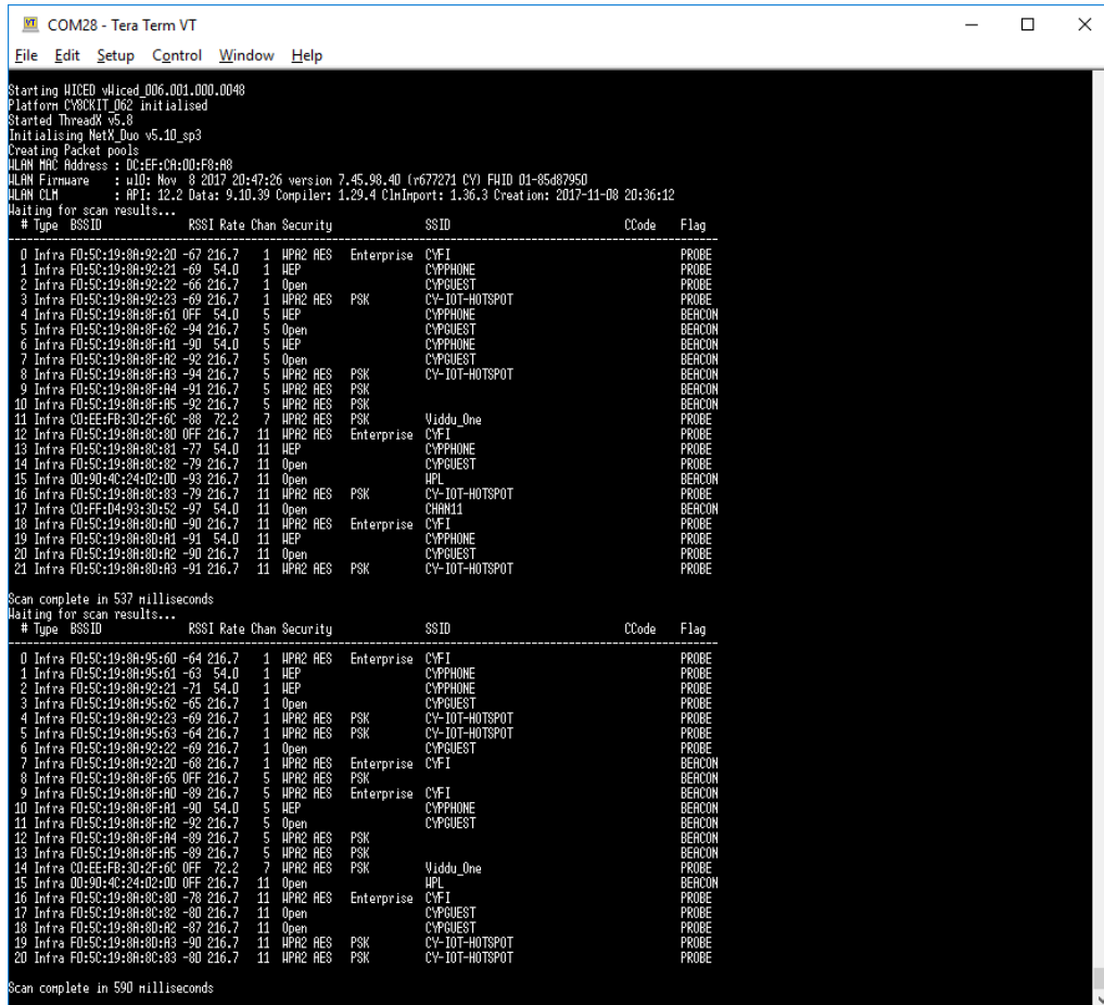
Figure 3-4. Console Output
