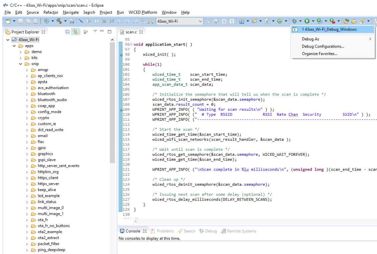
Figure 3-5. Debugging Project
