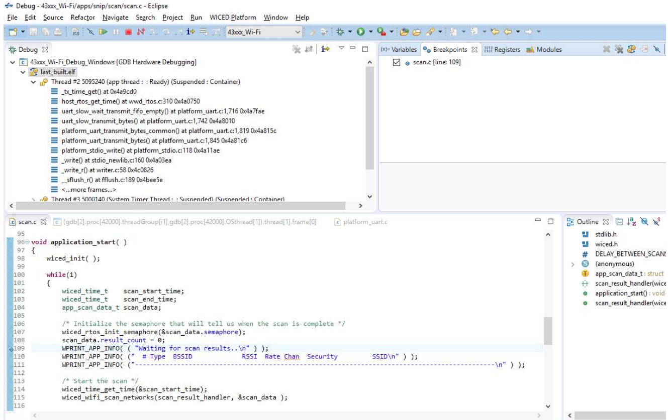
Figure 3-8. Enabling Breakpoint for Current Execution
