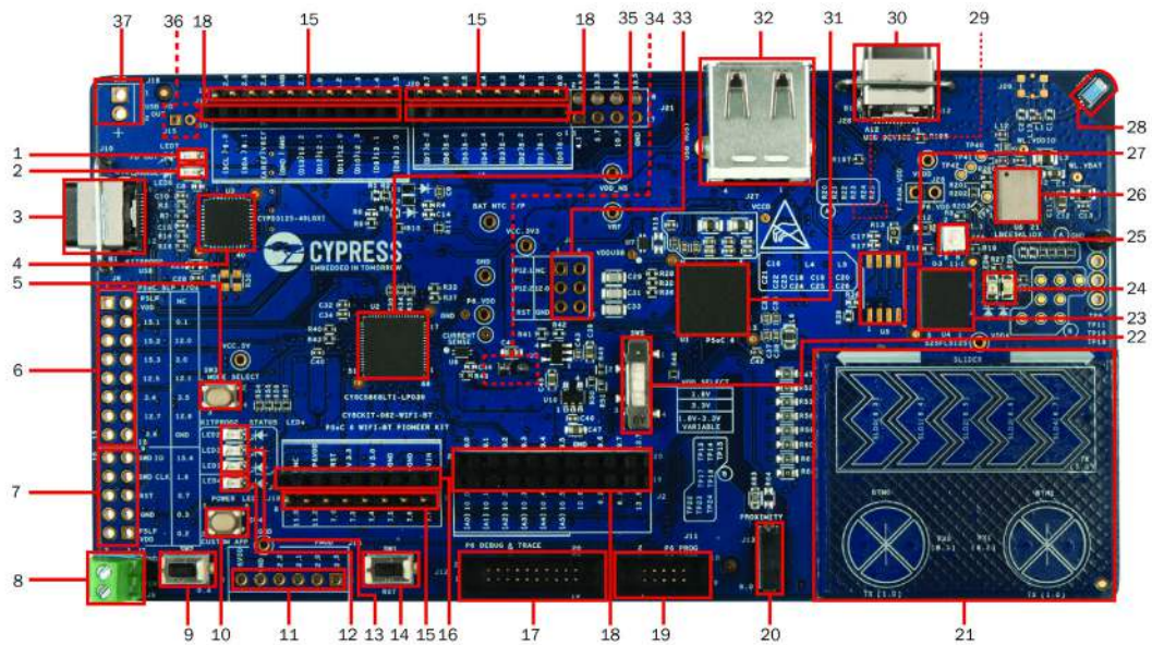
Figure 1-2. Pioneer Board
