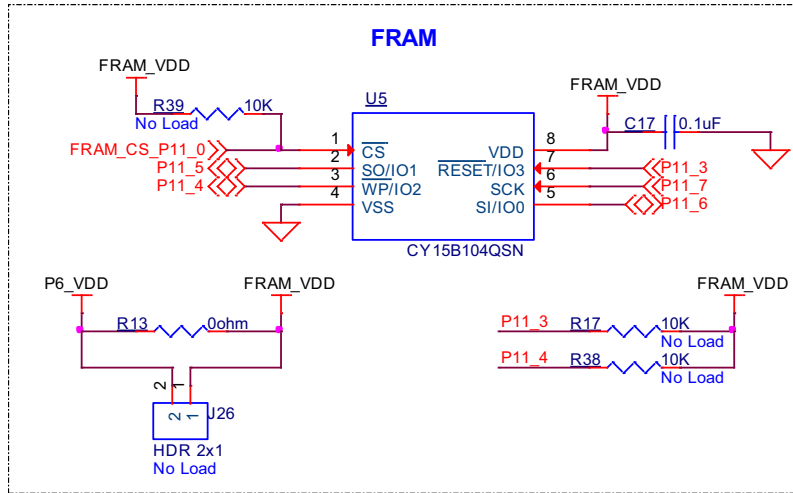
Figure A-8. Schematics of Cypress Quad SPI F-RAM
