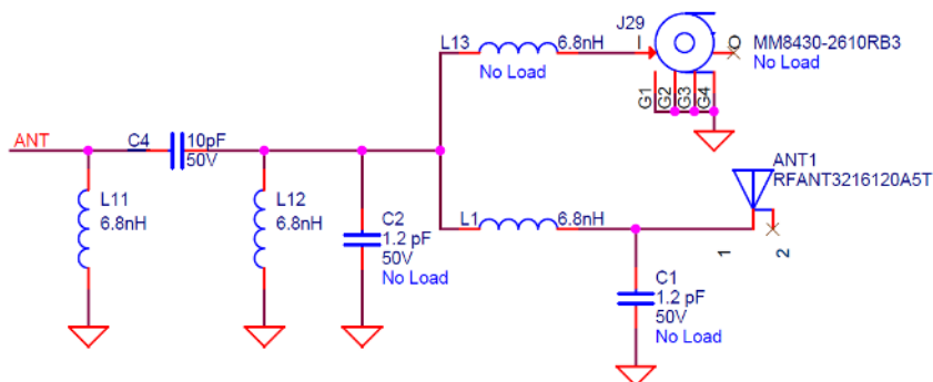
Antenna with Matching Network
