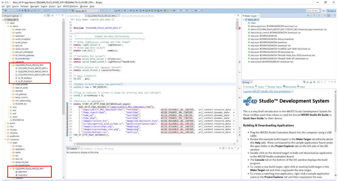
Figure 3-10. Setup Package in WICED Studio 6.1 (or later)
