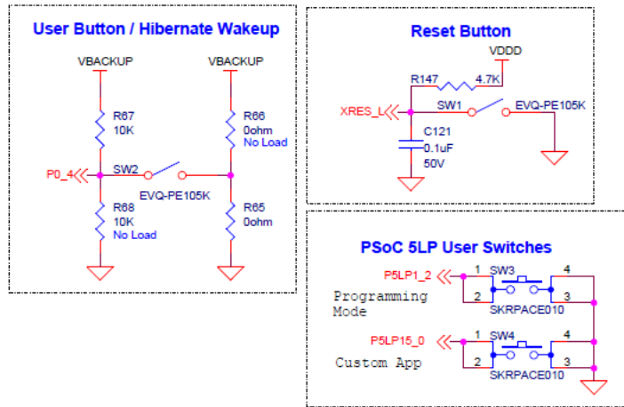
Figure A-6. Schematics of Push Buttons
