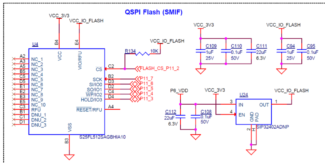
Figure A-7. Schematics of Cypress NOR Flash
