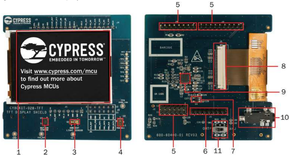
Figure 4-6. TFT Display Shield
