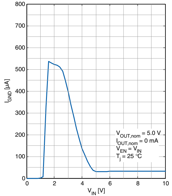
GND Current I_{GND} versus Input Voltage V_{IN}
