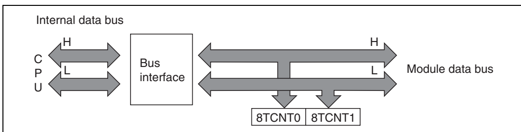
Figure 9.2 8TCNT Access Operation (CPU Writes to 8TCNT, Word)
