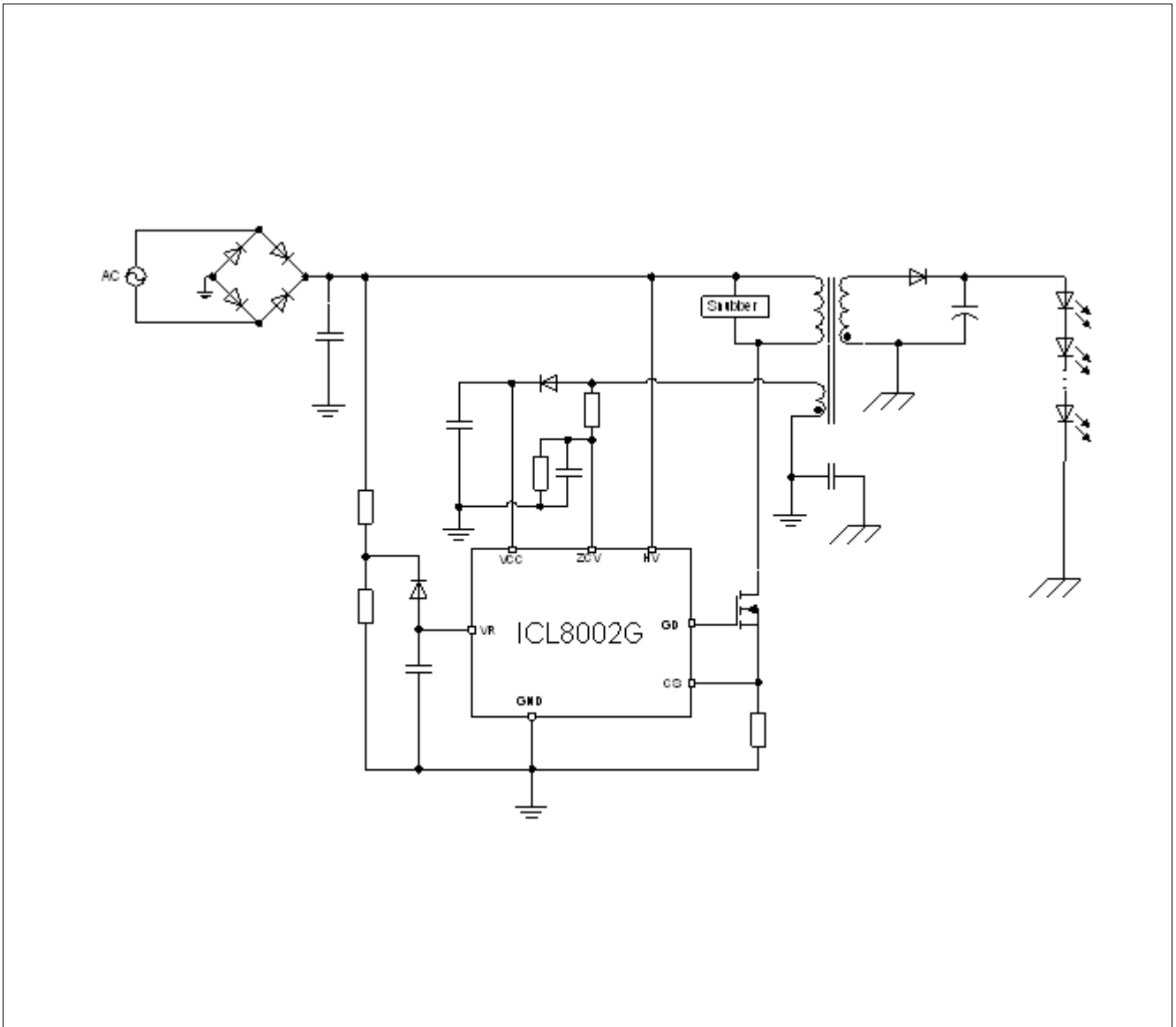
Figure 1 Application Circuit
