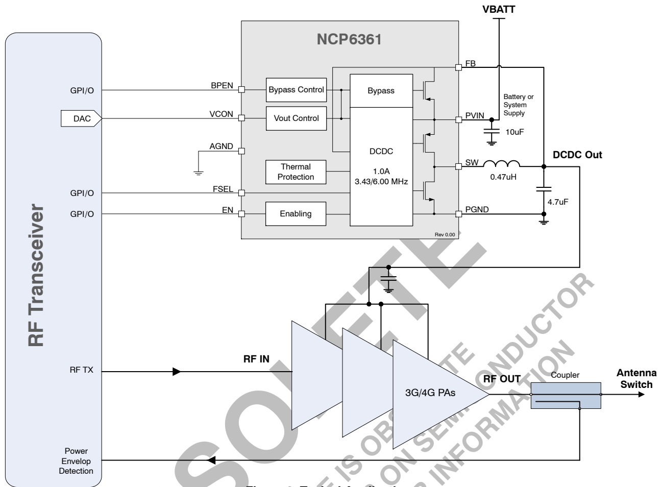
Figure 2. Typical Application
