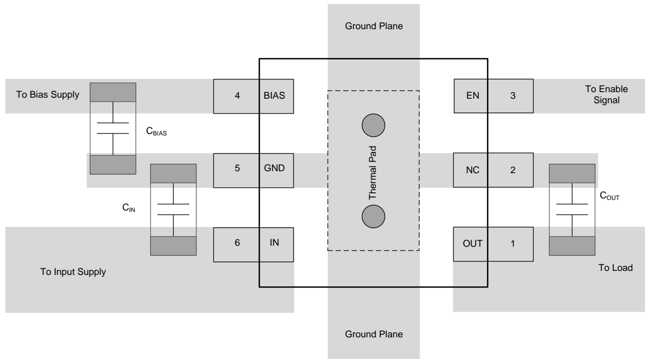
Figure 29. Recommended Layout
