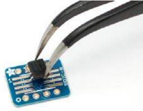
SMT Breakout PCB for SOIC-8, (/products/1212)
