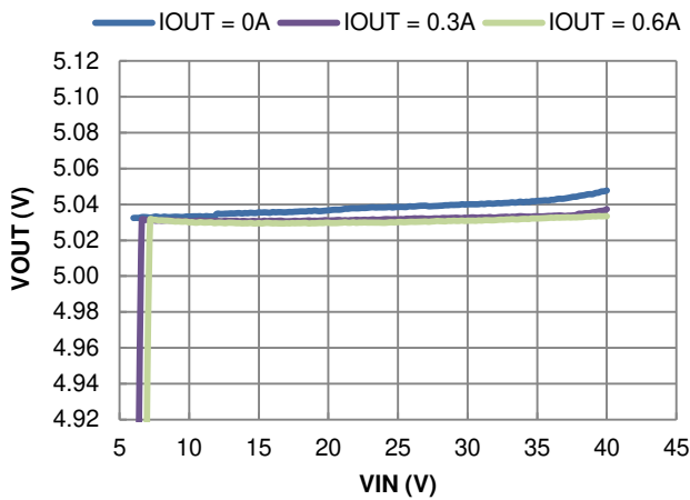
Figure 6. Line Regulation
