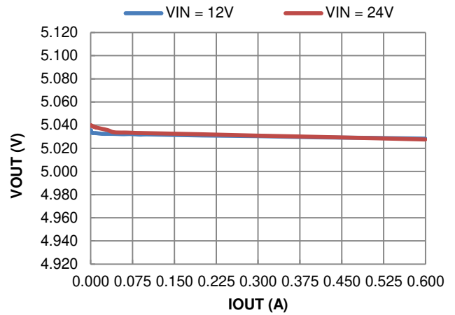
Figure 7. Load Regulation
