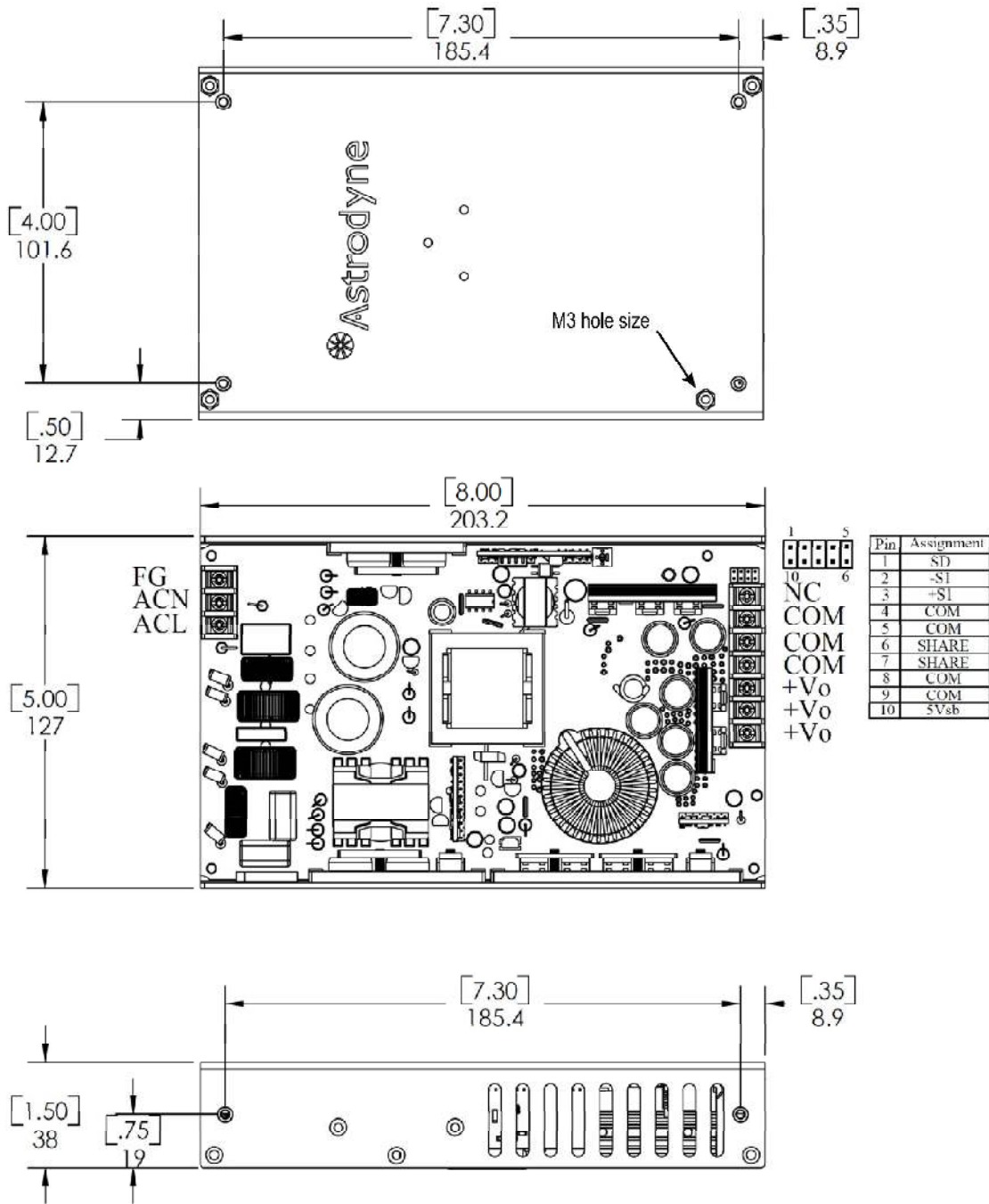
U-Bracket (PMK450S-xxU)
