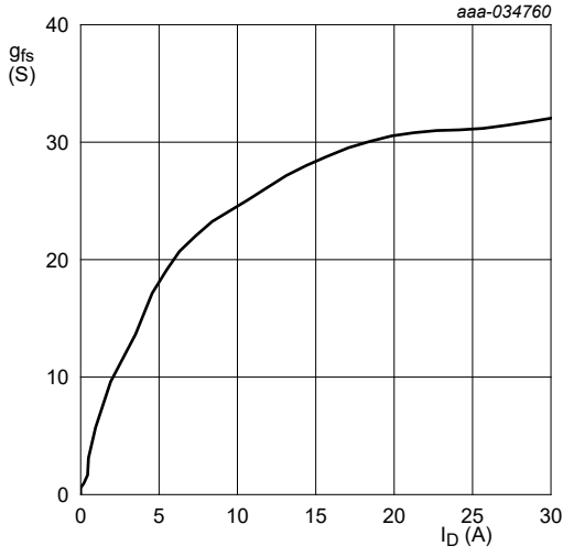
Fig. 17. Forward transconductance as a function of drain current; typical values
