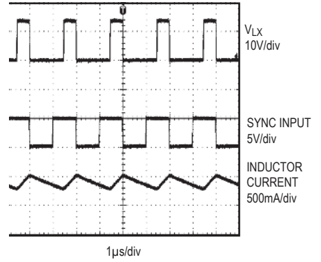
LX VOLTAGE, SYNC INPUT, AND INDUCTOR CURRENT MAX5096 toc21
