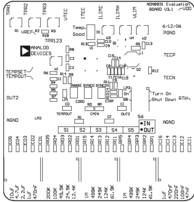
Figure 10. Top Layer Silkscreen
