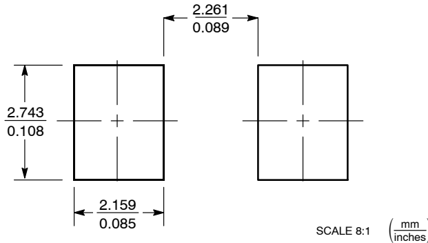
SOLDERING FOOTPRINT*
