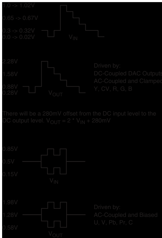
Figure 9. Typical Voltage Levels
