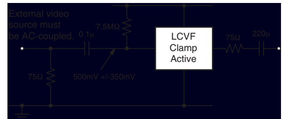
Figure 17. Biased SCART with AC-coupled Outputs
