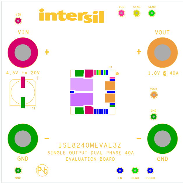
FIGURE 3. SILKSCREEN TOP
