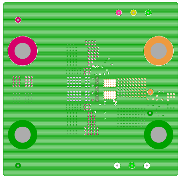
FIGURE 5. LAYER 2
