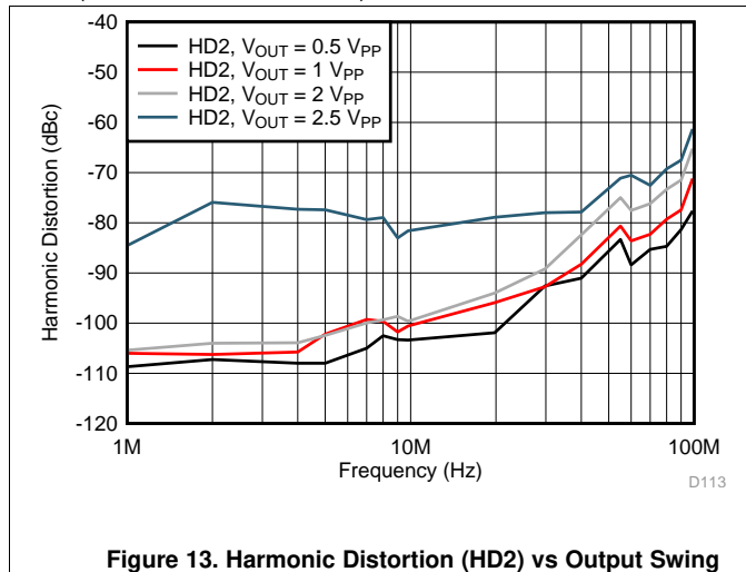
Figure 13. Harmonic Distortion (HD2) vs Output Swing
