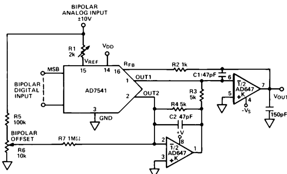
Figure 23. AD647 Used as DAC Output Amplifier
