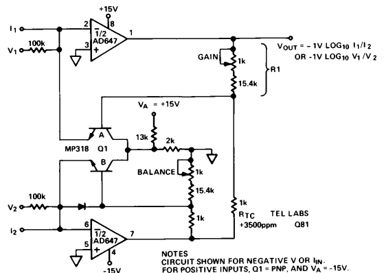
Figure 25. Log-Ratio Amplifier
