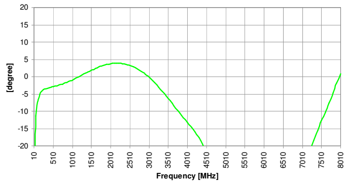
Phase Balance
