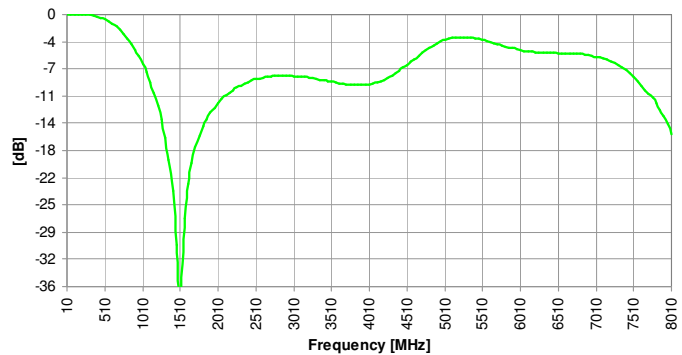
Return Loss-Input
