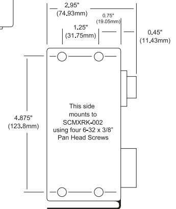
Figure 26: SCMXPRT-003/SCMXPRT-003 Physical Dimensions
