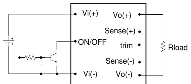
Figure 13: Remote On/Off Implementation
