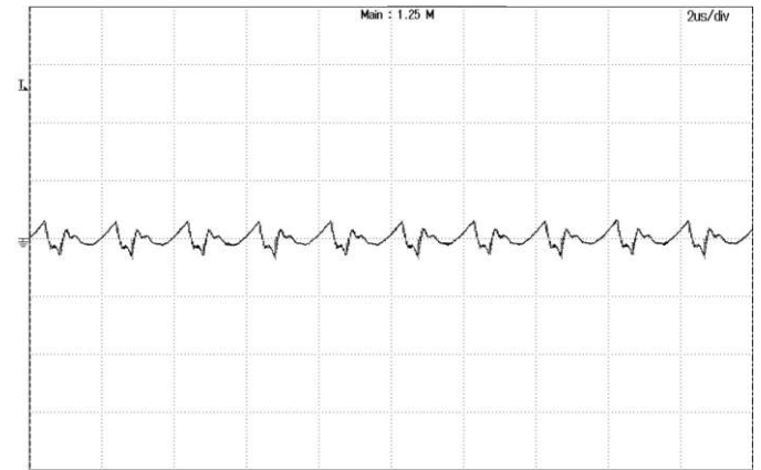
Figure 9: Input Terminal Ripple Current, i_c , at max output current and nominal input voltage with 12µH source impedance and 100µF electrolytic capacitor (500 mA/div, 2µs/div).
