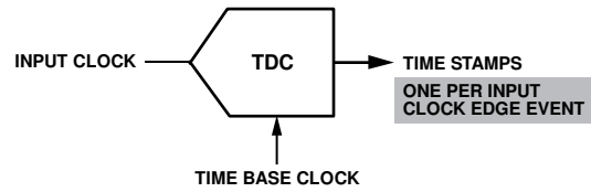
Figure 92. TDC Diagram
