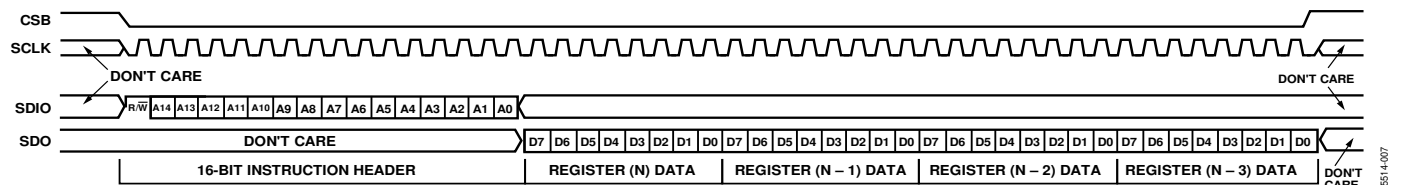
Figure 123. Serial Control Port Read—MSB First, Address Decrement, Four Bytes of Data
