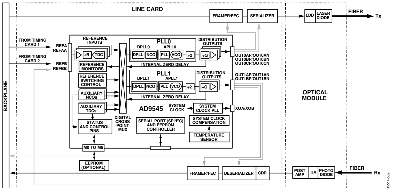
Figure 116. Optical Line Card Loop Timing Example
