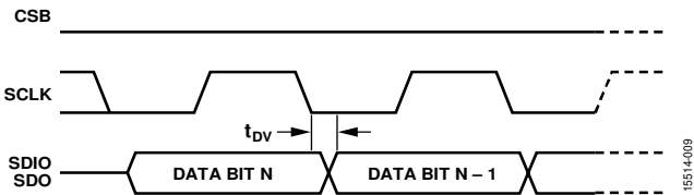
Figure 125. Timing Diagram for Serial Control Port Register Read—MSB First
