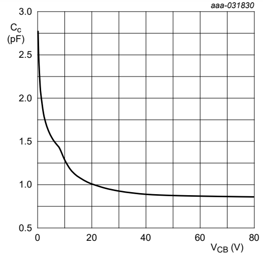
Fig. 21. NHDTC114YT: Collector capacitance as a function of collector-base voltage; typical values
