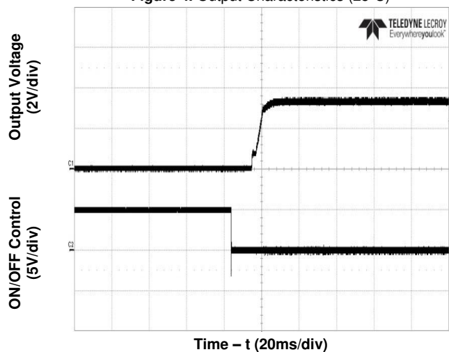
Figure 6. Start-Up from Enable Control (typical Vin, full load, no external output capacitor)
