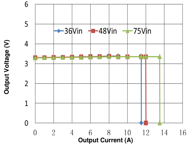
Figure 4. Output Characteristics (25°C)
