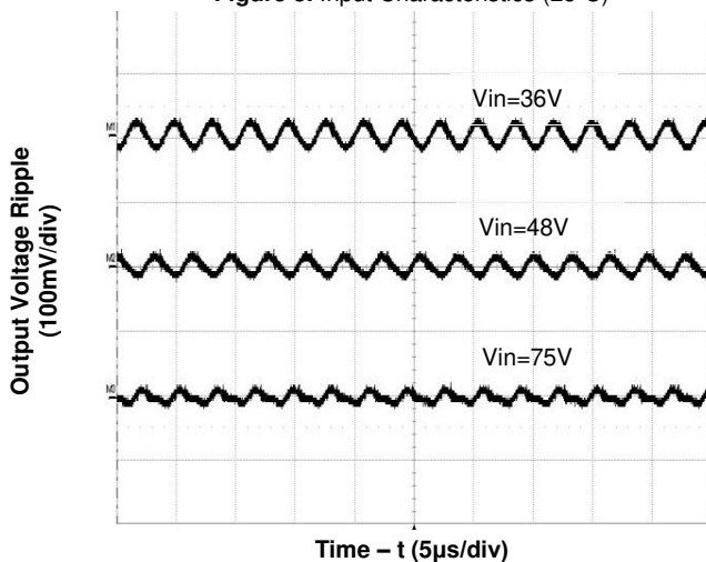
Figure 5. Output Ripple Voltage at Full Load (tested with no external output capacitor)
