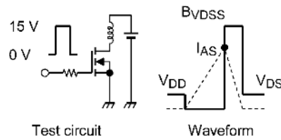
Fig. 9.16 Test Circuit/Waveform
