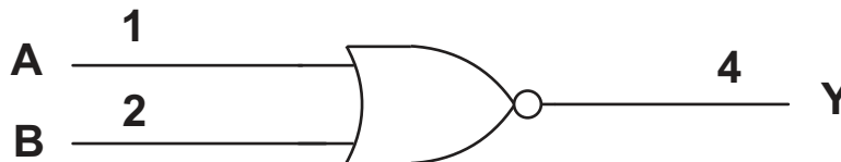
Figure 9-1. Logic Diagram
