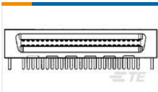
TE Part #5-5175474-7 .050CL,CHAMP,R/TANG RCPT,60POS
