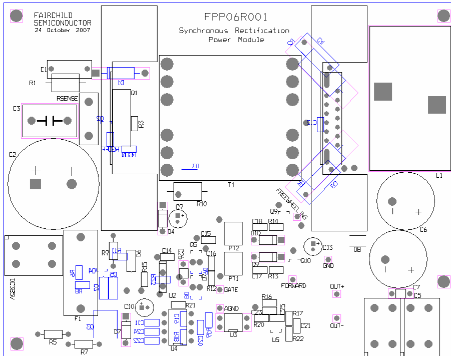
< Component assembly >
